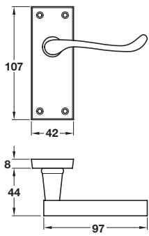
901.98.891 Lever latch handle
