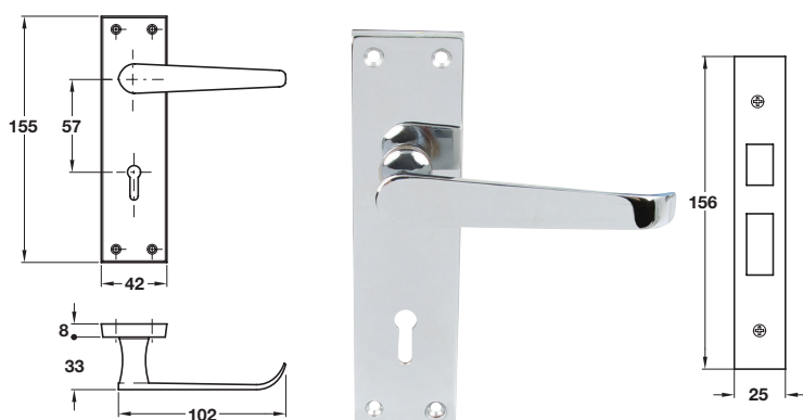
901.98.888 Lever lock handle
