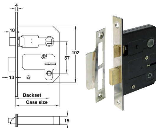
911.02.304 Mortice bathroom lock
