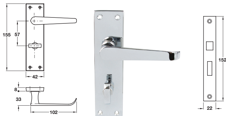
901.98.890 Lever bathroom handle
