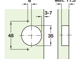
Drilling dimensions for cup fixing Drilling pattern 48/6
