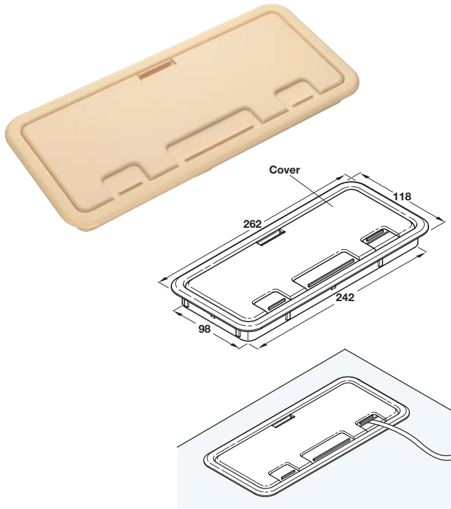
A Rectangular cable outlet, 98 x 242 mm
