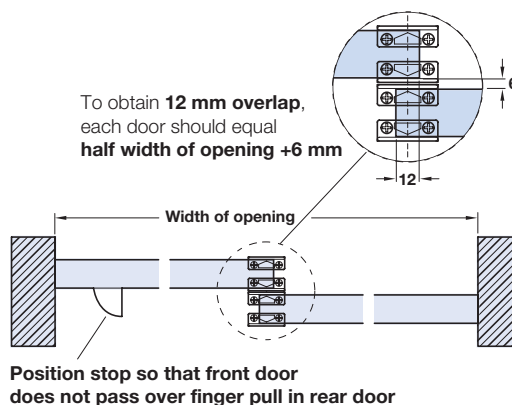
Two doors - one sliding to each side of opening, both doors on a single track
