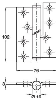
Falling hinge Anti-clockwise closing shown
