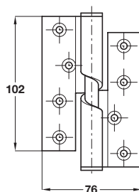
Rising hinge Anti-clockwise closing shown
