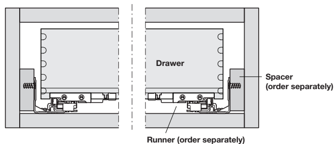
Installation dimensions of drawer
