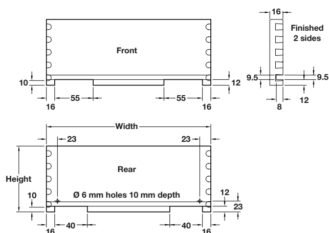
Installation dimensions of drawer
