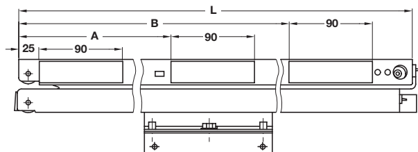
Installation dimensions
