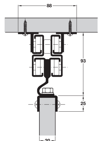
Installation
