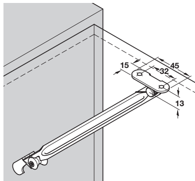
Side panel mounting fixing method
