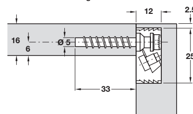
Recommended drilling for 16 mm board thickness
