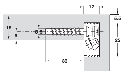
Recommended drilling for 19 mm board thickness
