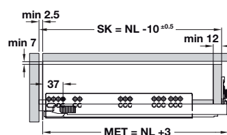
Inset Drawer
