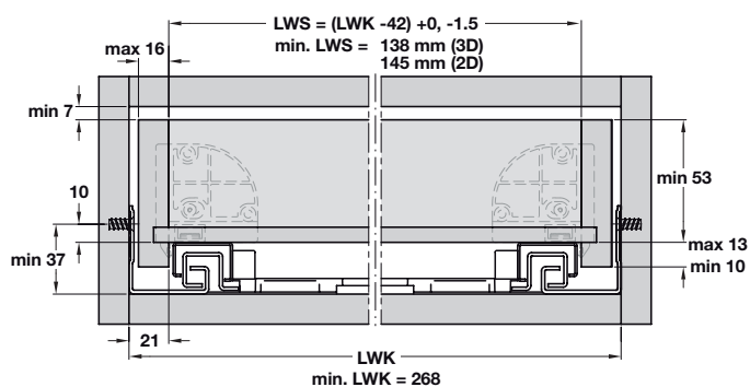
Installation dimensions of drawer
