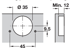
Drilling pattern for cup fixing
