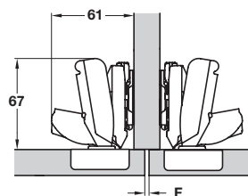
Drawing show application on 0 mm thick mounting plate
