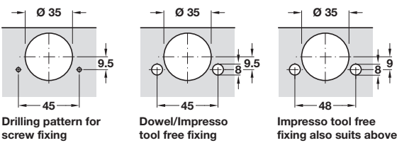
Drilling pattern for cup fixing
