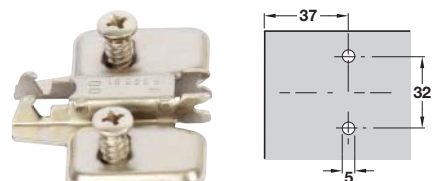
With pre-mounted Euro screws
