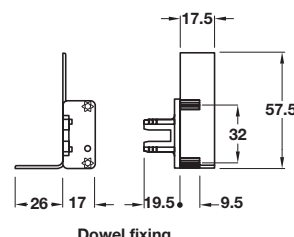
Dowel fixing
