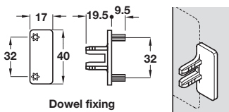
Dowel fixing
