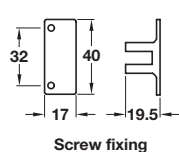
Screw fixing
