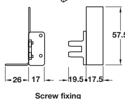
Screw fixing
