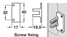
Screw fixing
