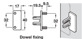
Dowel fixing
