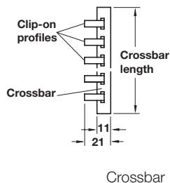
Quantity of clip-on profiles, determined by length of cross bar
