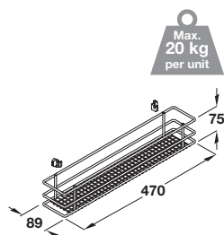
150 mm cabinets - order frame separately
