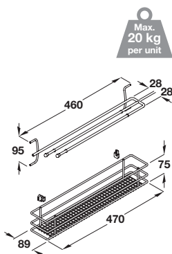
150 mm cabinets - order frame separately
