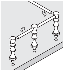
Posts press fit into Ø 6 mm, 12.5 mm deep holes
