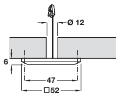
Loox 12V LED 2010 RGB colour change light, 52 mm
