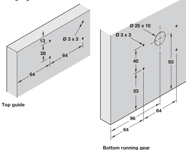
Drilling diagram
