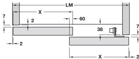
Door overlap
