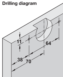
Drilling diagram
