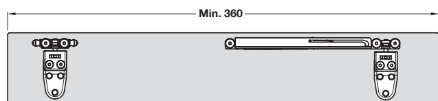
Minimum door width with one soft closing mechanism
