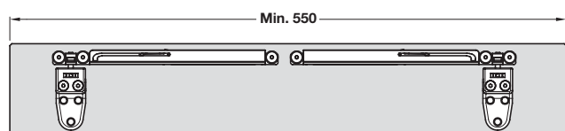
Minimum door width with two soft closing mechanism
