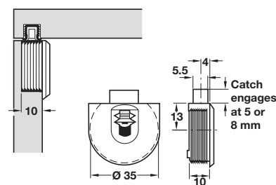
Alternative top guide F with channel recessed
