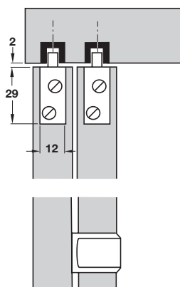
Top guide B with channel recessed
