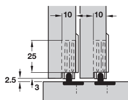
Bottom guide D with track recessed
