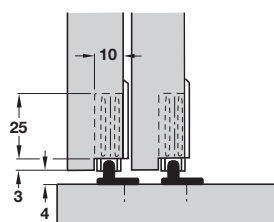
Bottom guide D with track surface fixed
