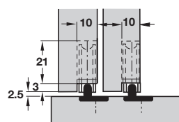
Alternative bottom guide G with track recessed
