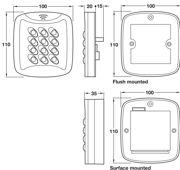
Flush mounted
