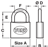
Standard shackle
