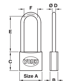
Long shackle
