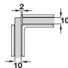
Glass machining without miter, 10 mm glass
