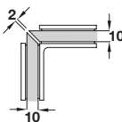
Glass machining with 45° miter, 10 mm glass
