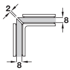
Glass machining with 45° miter, 8 mm glass
