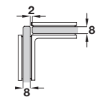
Glass machining without miter, 8 mm glass
