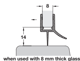
when used with 8 mm thick glass
