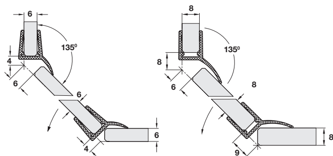
when used with 6 mm thick glass
