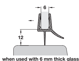
when used with 6 mm thick glass
