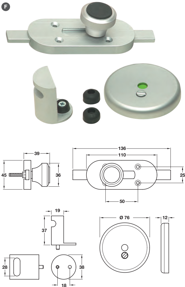
Door drilling detail for indicator bolt set
