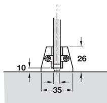
Bottom guiding with floor guide H
