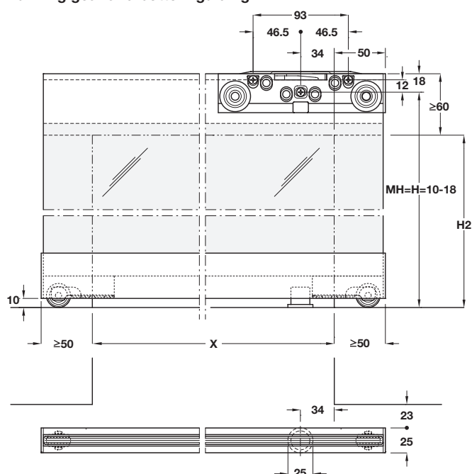
Running gear and bottom guiding
