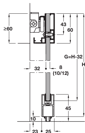
Bottom guiding on hard floor G = Glass height
