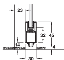
Bottom guiding on soft floor with running track
