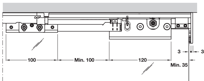
Section trolley hanger 50 kg with soft closing mechanism
