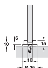
Floor guide with zero clearance
