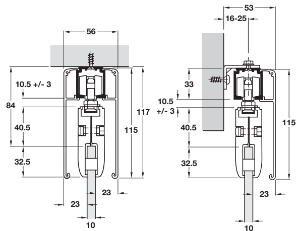
Ceiling installation
