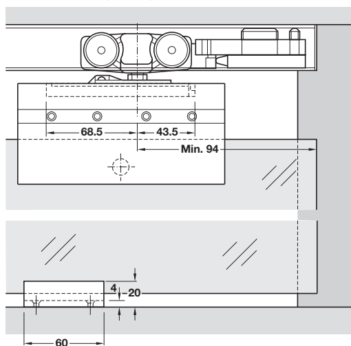
Section trolley hanger and guide
