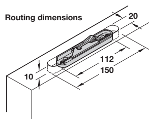
Routing dimensions
