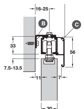
Wall mounting with clip panel and concealed mounting bracket
