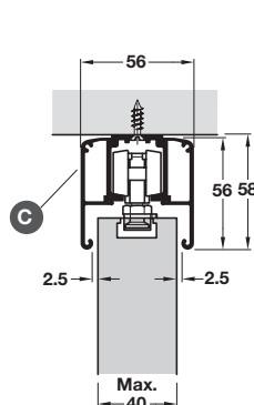
Ceiling installation with clip panel
