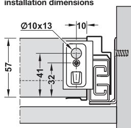
Rear wooden panel installation dimensions
