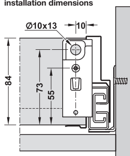
Rear wooden panel installation dimensions
