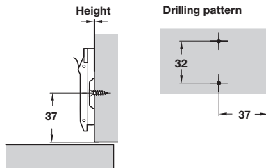
Drilling pattern
