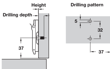
Drilling pattern
