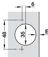
Drilling pattern
