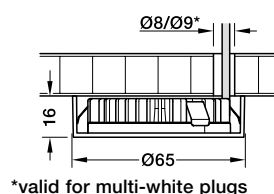
833.72.124 Round version bezel
