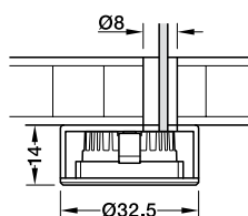
Surface mounting, round
