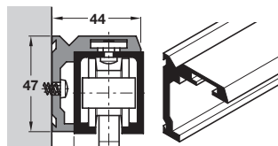
940.80.253 - Side fixing profile, 2.5 m length
