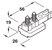
940.42.041 - Additional track buffer
