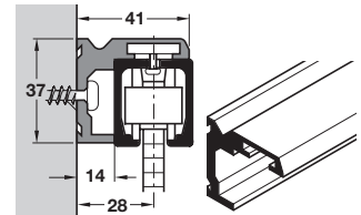
940.40.203 - Side fixing profile, 2.0 m length
