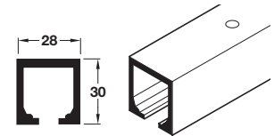
940.40.200 - Single top track, 2.0 m length
