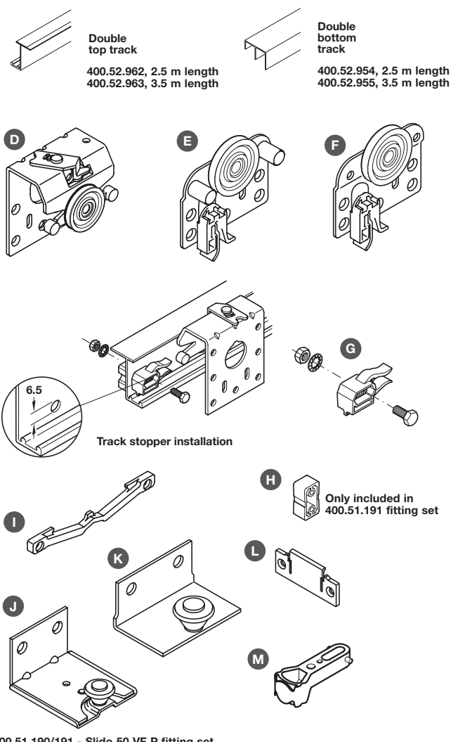
400.51.190/191 - Slido 50 VF P fitting set
