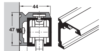
940.80.253 - Side fixing profile, 2.5 m length
