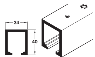
940.80.200 - Single top track, 2.0 m length
