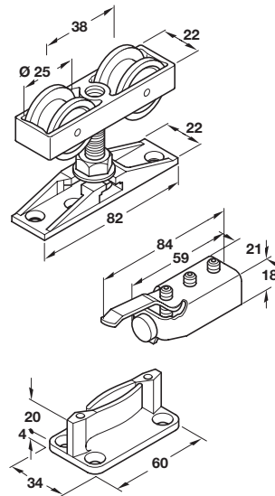
940.40.001 - Fitting set
