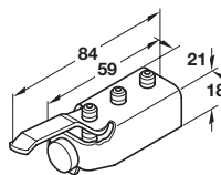
940.40.041 - Additional track stopper
