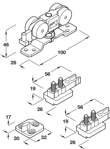
941.02.119 - Fitting set
