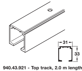
940.43.921 - Top track, 2.0 m length
