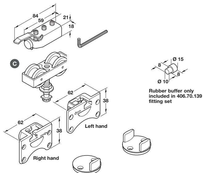
406.70.120/139 - Hawa-Dorado fitting set
