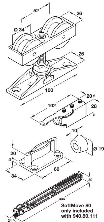
940.80.001/111 - Fitting sets
