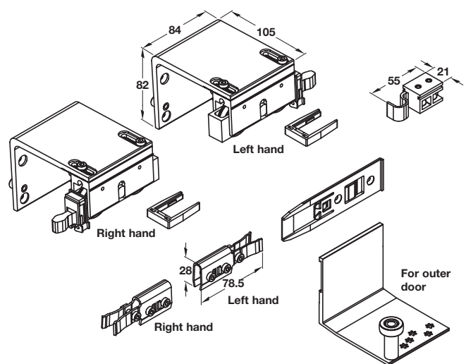
405.35.101 - Outer door fitting set
