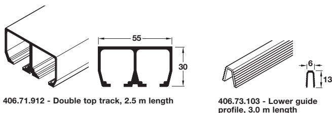
406.70.120/139 - Hawa-Dorado fitting set
