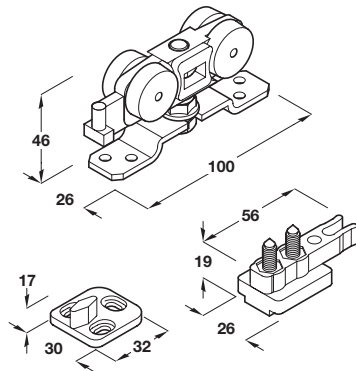
940.60.006 - Fitting set
