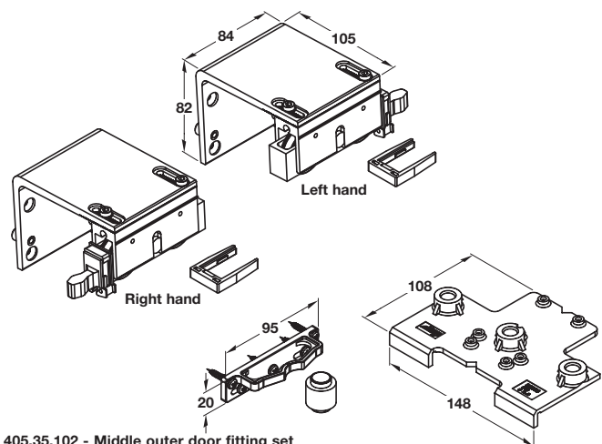
405.35.102 - Middle outer door fitting set
