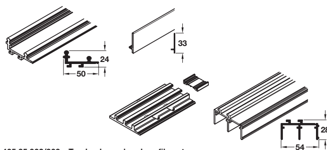
405.35.902/903 - Track, channel and profile set
