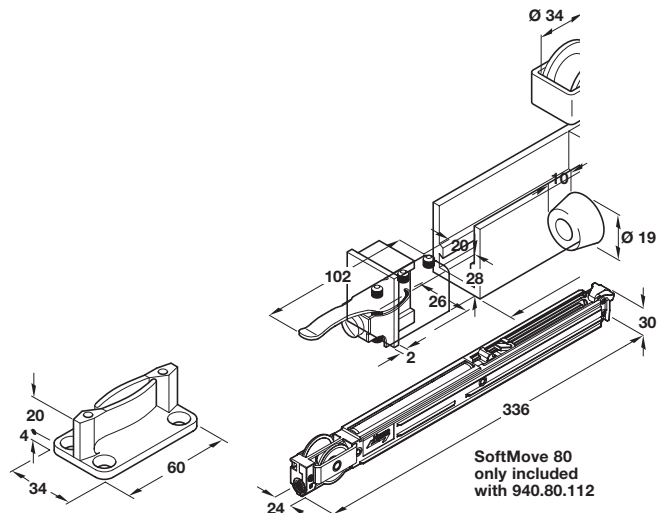
940.80.002/112 - Fitting sets
