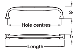
Pull handle
