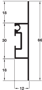
Horizontal/vertical can be used for drawer application (horizontal shown)
