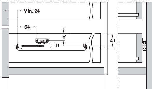
Installation For roller and ball bearing runners
