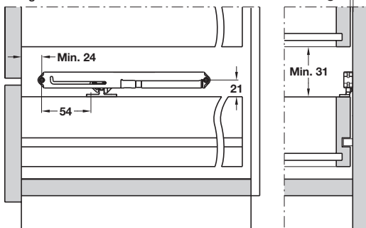
For groove mounted runners
