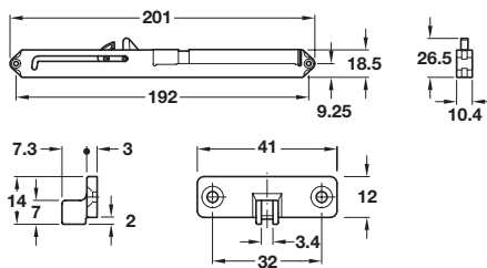
Installation For roller and ball bearing runners
