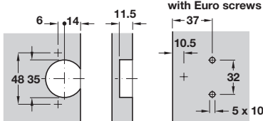
Drilling pattern 48/6
