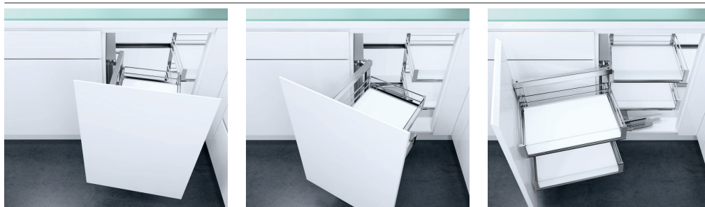
Automatic pull-out action - rear baskets automatically follow front baskets when the door is pulled
