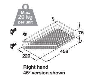
Angled 300 mm cabinet - order frame separately
