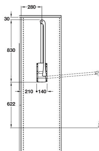
Installed in middle of cabinet side wall
