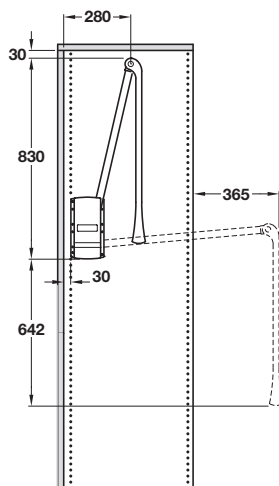
Installed at rear using series drilled holes
