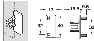
Dowel fixing
