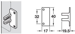
Screw fixing
