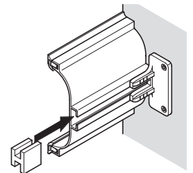
Screw fixing profile connector
