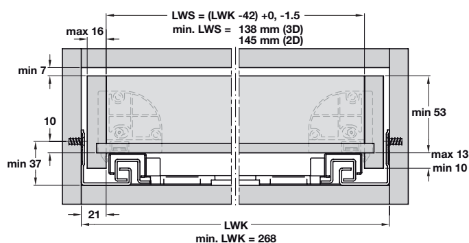
Installation dimensions of drawer
