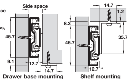
Drawer base mounting
