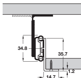
Keyboard shelf mounting
