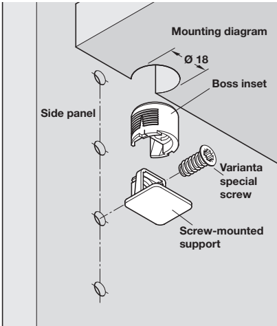
TAB shelf connectors consisting of: support and boss insert without tensioning element
