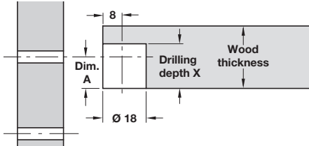
TAB shelf connectors consisting of: support and boss insert without tensioning element
